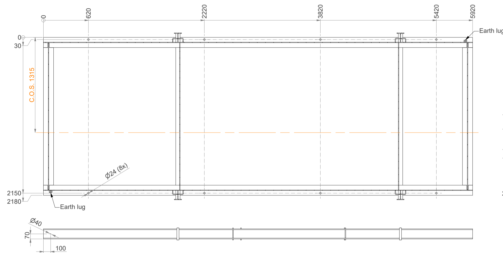
A-A ( 1 : 25 ) section view of foundation holes
