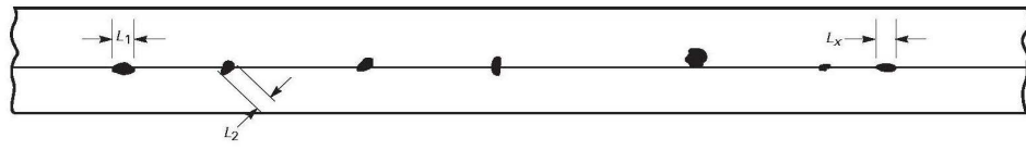
Figure 4-1 Aligned Rounded Indications
