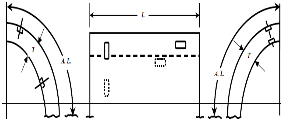
Figure 1 – ASME Calibration Block - Pipe Welds
