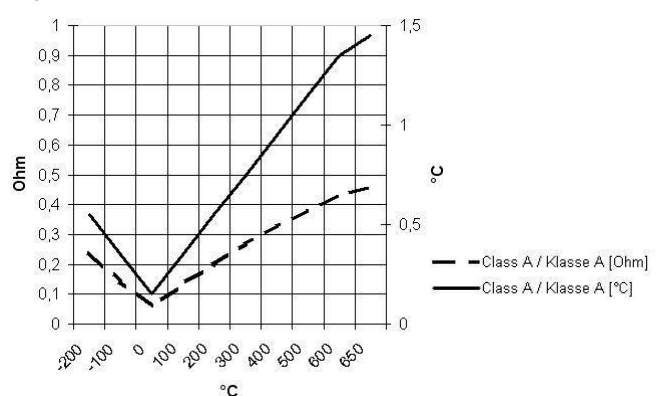
Figure 2: Deviation limit (IEC 60751) Class A
