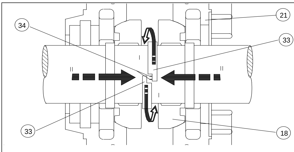
Illustration 7: Installation of the loose oil ring
