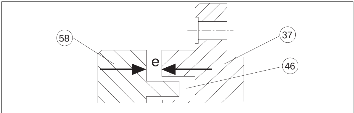
Illustration 13: Clearance between dust flinger and seal carrier
