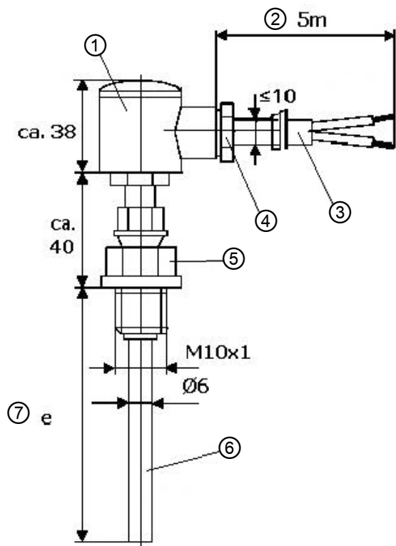
Figure 8: Resistance thermometer
