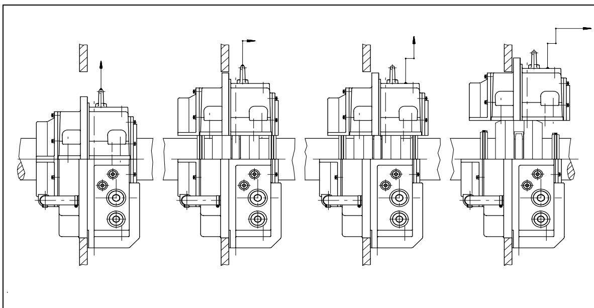
Illustration 2: Dismantling of the housing - top half
