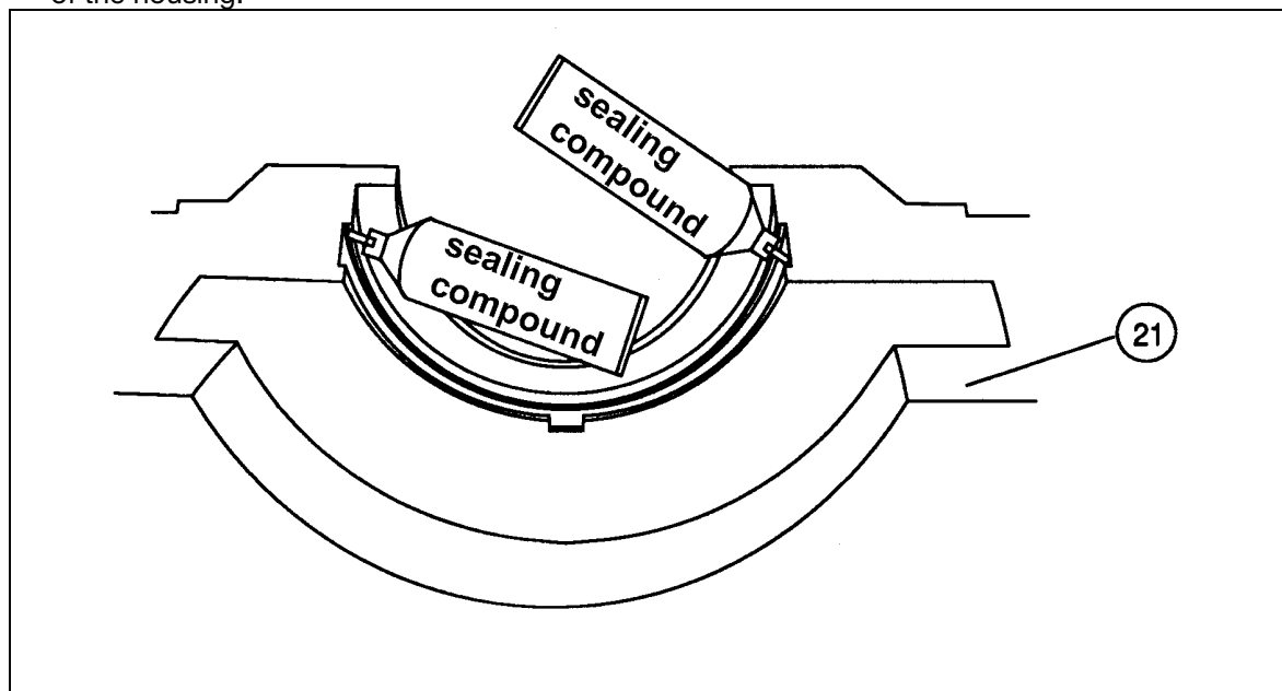
Illustration 4: Application of sealing compound to the integrated seal groove
