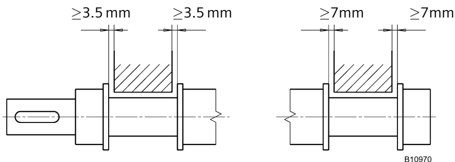
Floating bearing DE
