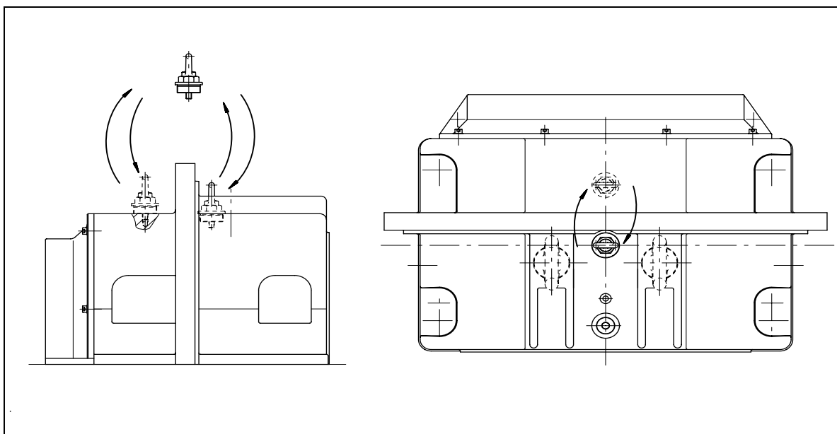
Illustration 1: Assembly device
