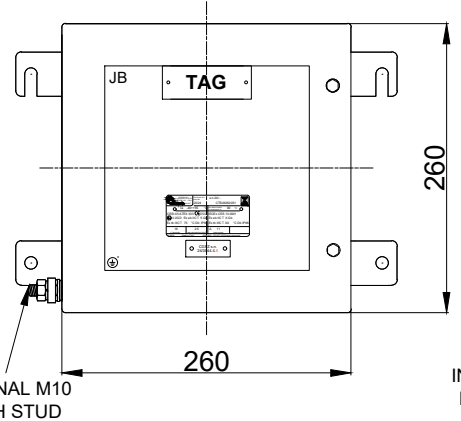
EXTERNAL VIEW
