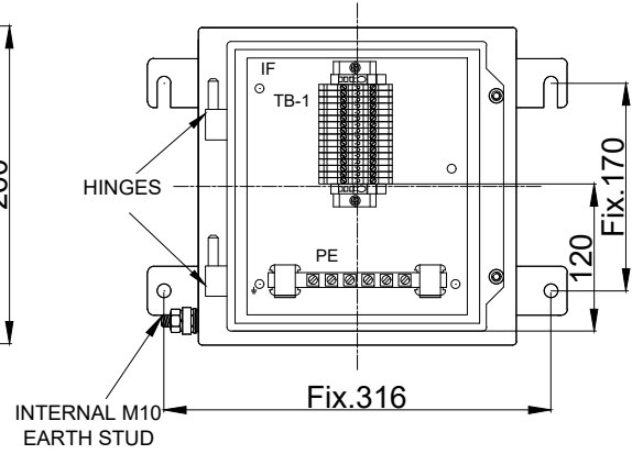
INTERNAL VIEW
