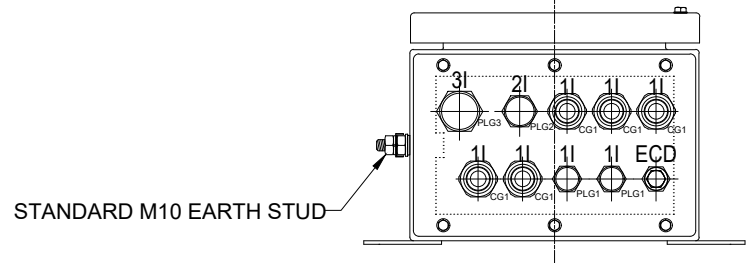
RIGHT SIDE
